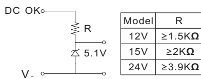
(a) 5V signal
