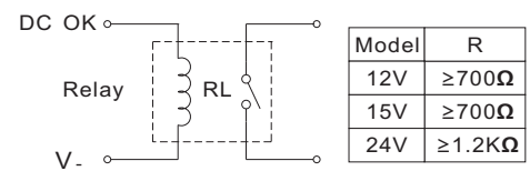
(c) Relay
