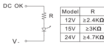
(b) LED
