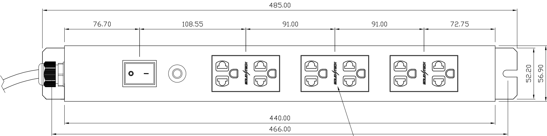
Top View
