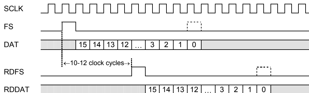
Figure 6 FSB Operation
