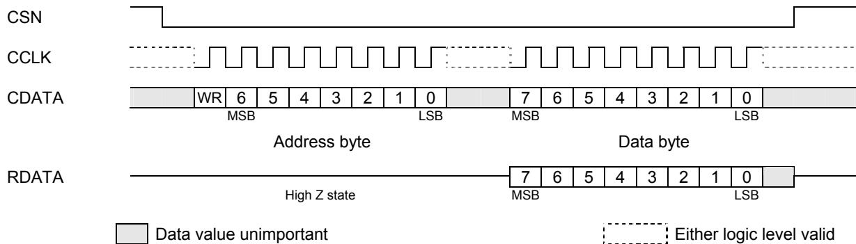
Figure 7 C-BUS Operation
