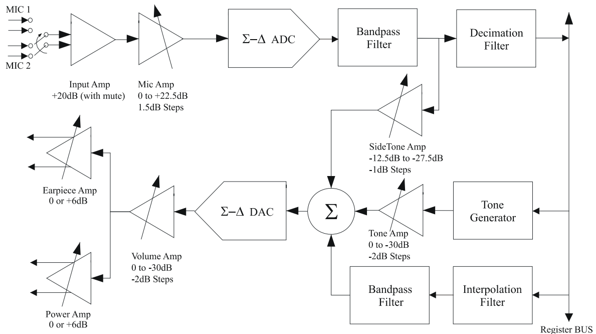
Figure 4 Voice Codec Block Diagram
