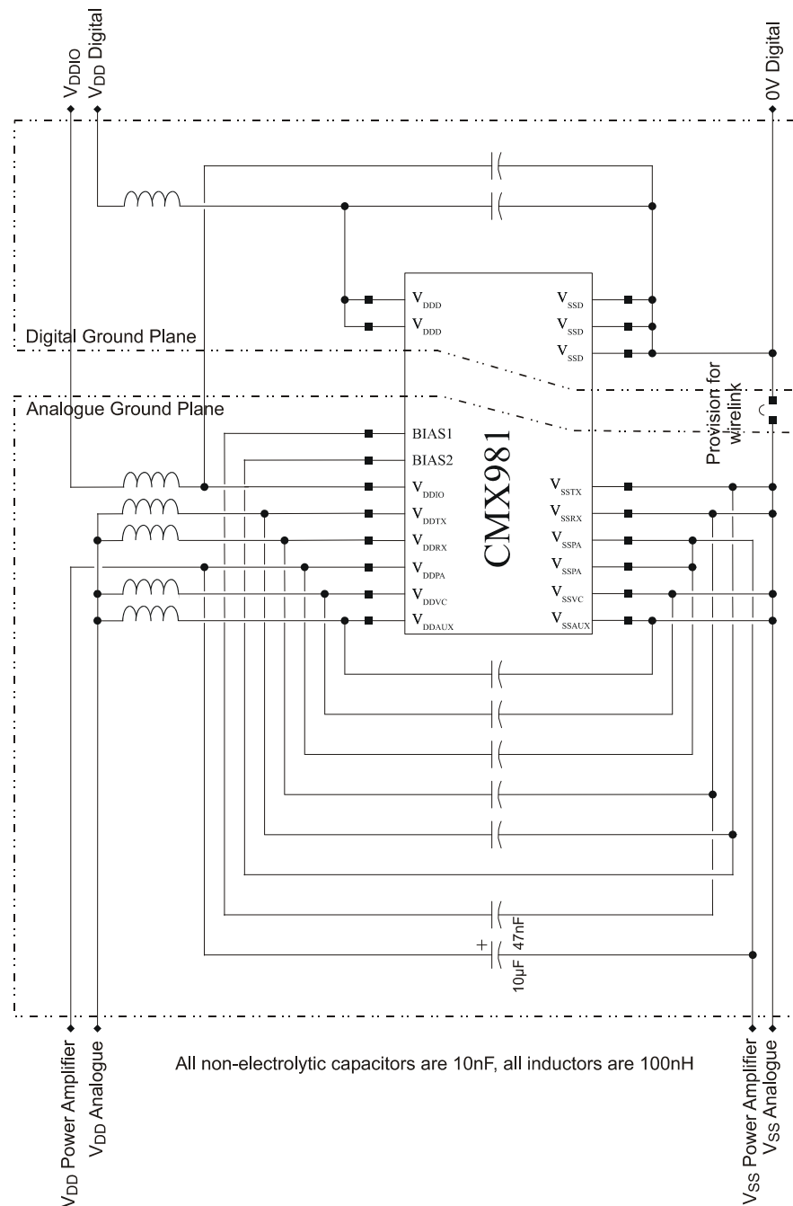
Figure 3 Recommended External Components
