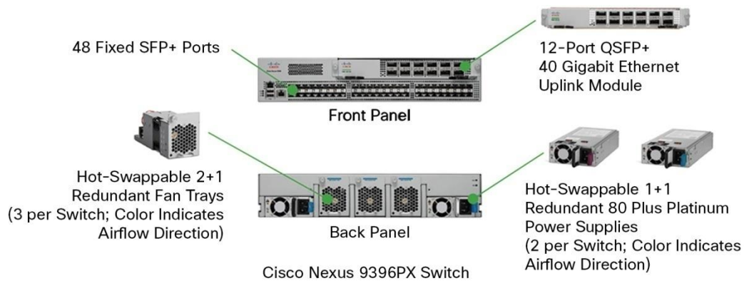
Figure 8. Cisco Nexus 9300 Platform Components
