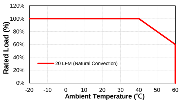
TRG36A Derating Curve
