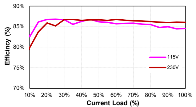
TR18RDM090 (Eff Vs Io)
