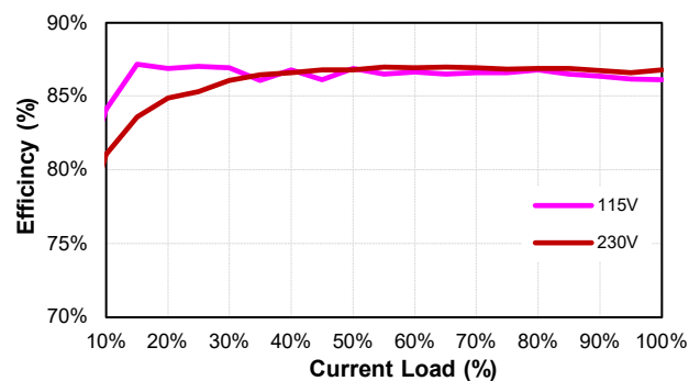
TR18RDM150 (Eff Vs Io)
