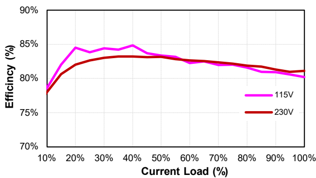
TR18RDM050 (Eff Vs Io)
