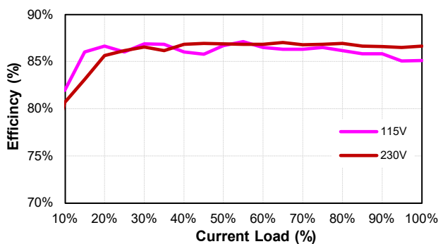
TR18RDM120 (Eff Vs Io)
