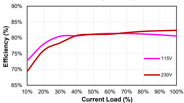
CFM40T-05 (Eff Vs Io)
