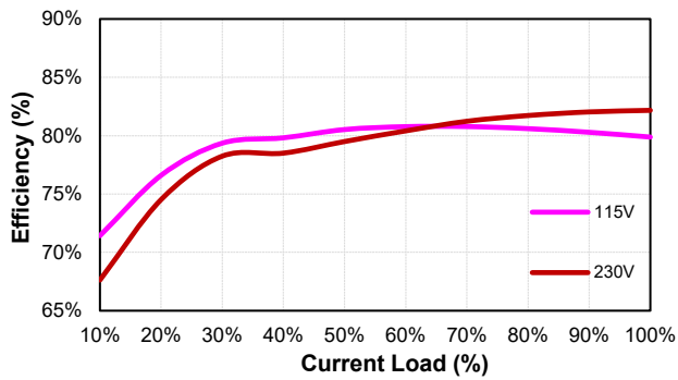
CFM40T-03 (Eff Vs Io)
