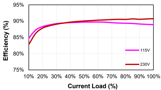
CFM36SX150 (Eff Vs Io)
