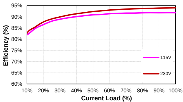
CFM150S480 (Eff Vs Io)
