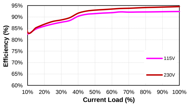
CFM150S280 (Eff Vs Io)
