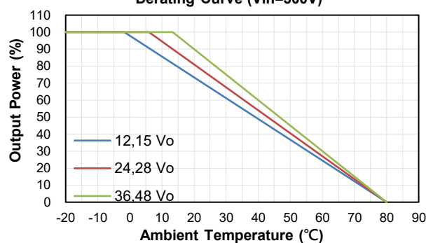
CFB750-300S CMFD+HS(HD) Derating Curve (Vin=300V)
