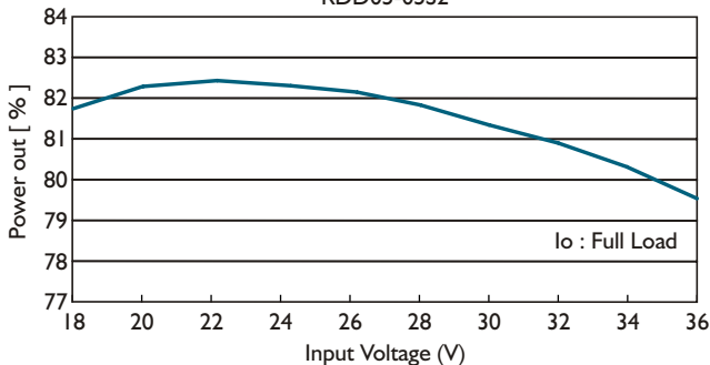
Efficiency Vs Input Voltage RDD05-05S2
