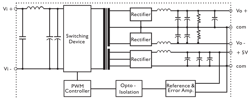
Block diagram for KDD25 series with triple output
