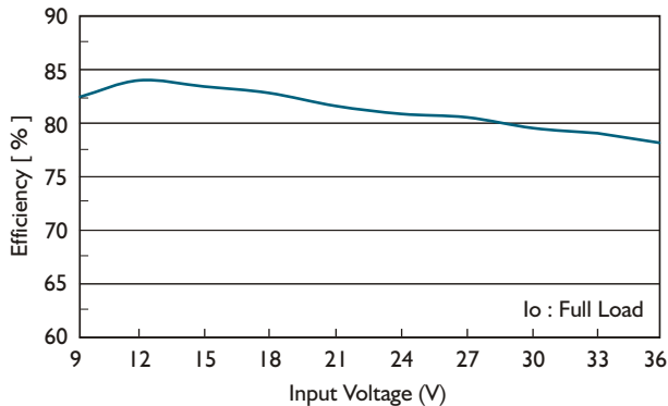
Efficiency Vs Input Voltage IDD10-05S4U
