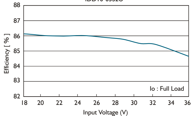
Efficiency Vs Input Voltage IDD10-05S2U
