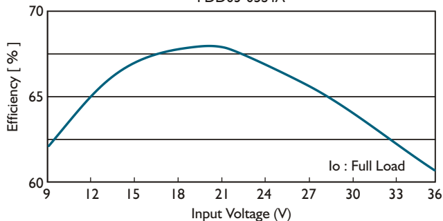
Efficiency Vs Input Voltage FDD03-05S4A
