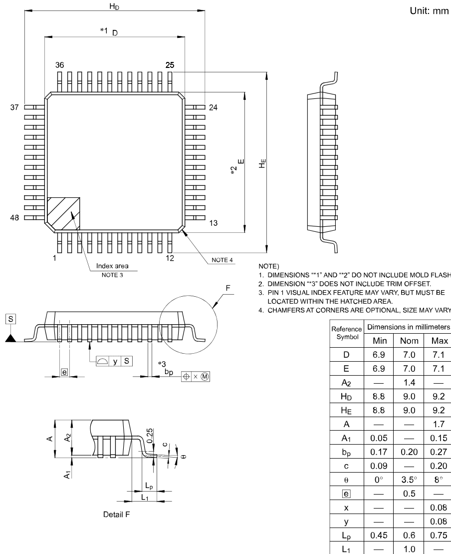
Figure 26 - LQFP48 Package
