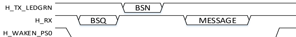
Figure 6: UART-SHTP - Sending a message to the FSP201
