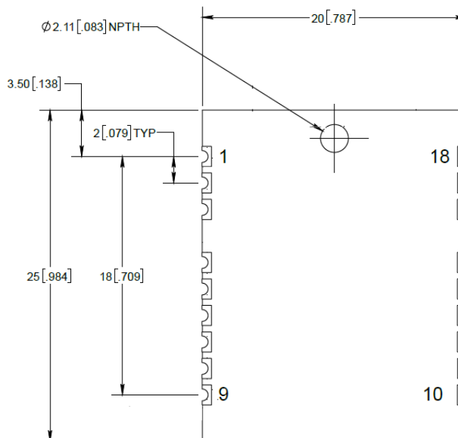
Figure 2-3: FSP201 Module Dimensions (Component side)
