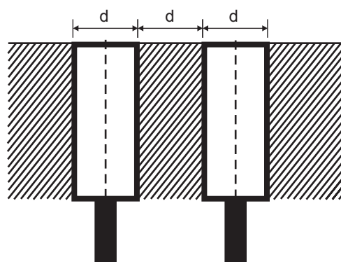
Fig. 18 Flush sensors, when installed together in damping material
