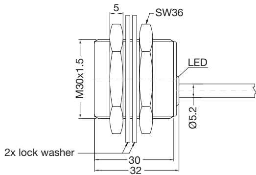
Fig. 29 Short body, flush version, cable
