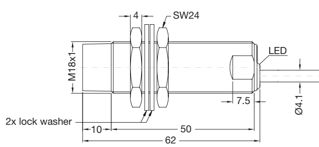
Fig. 26 Long body, non-flush version, cable
