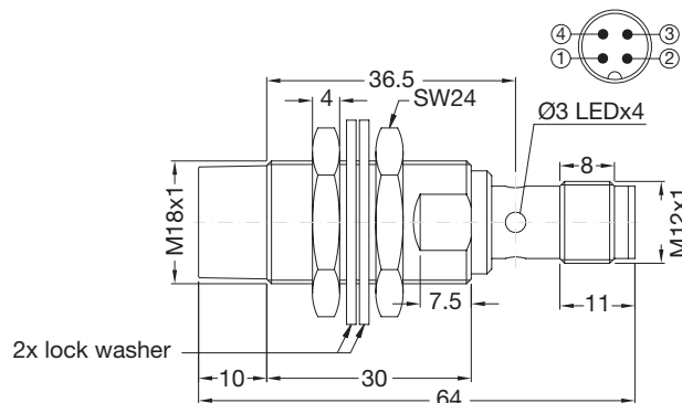
Fig. 24 Short body, non-flush version, plug
