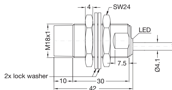
Fig. 22 Short body, non-flush version, cable
