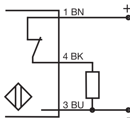
Fig. 6 PNP - Normally closed
