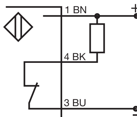
Fig. 4 NPN - Normally closed
