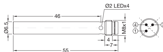
Fig. 10 Long body, flush version, plug
