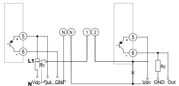
Open collector output
