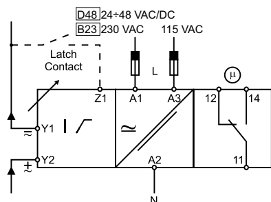
Fig. 3 Direct connection
