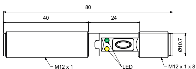
Fig. 8 Plug CA12CAF...M1IO
