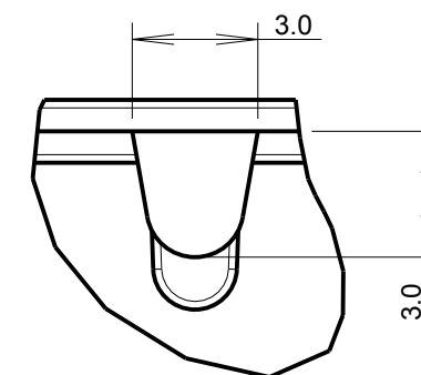
DETAIL A GATE CROSS-SECTION SCALE 5:1
