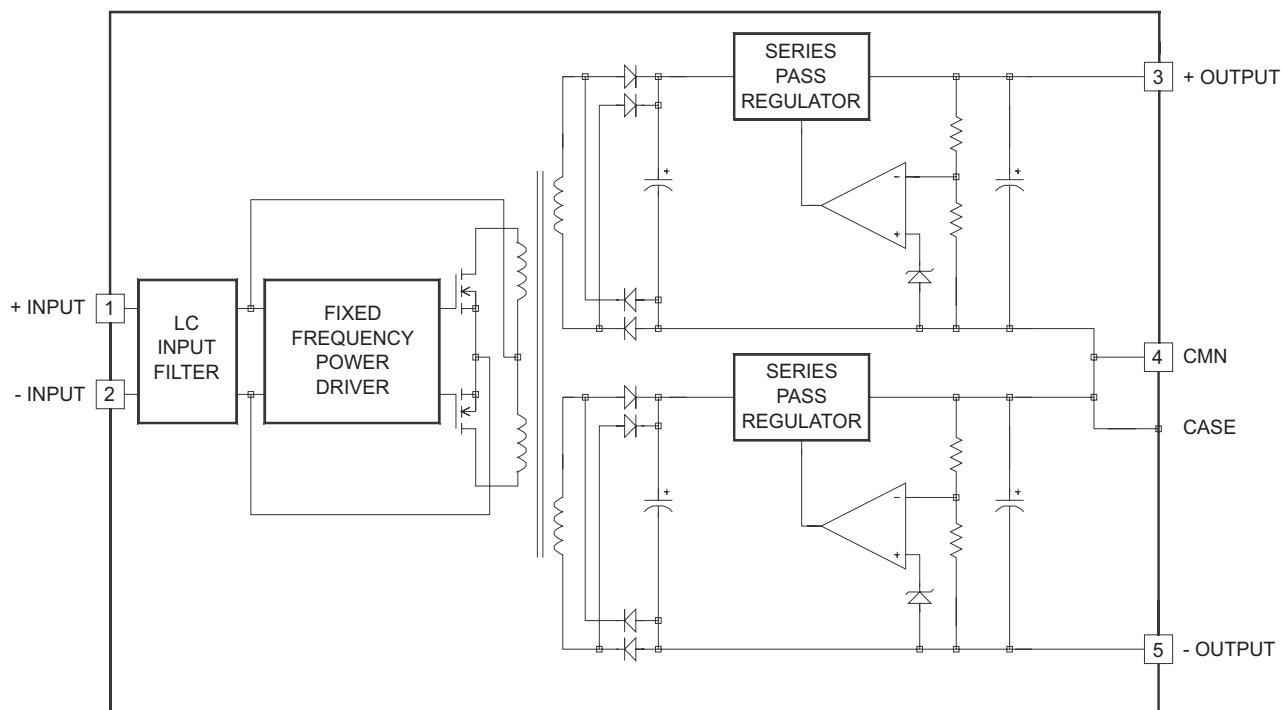
5 Watt Dual Series Block Diagram
