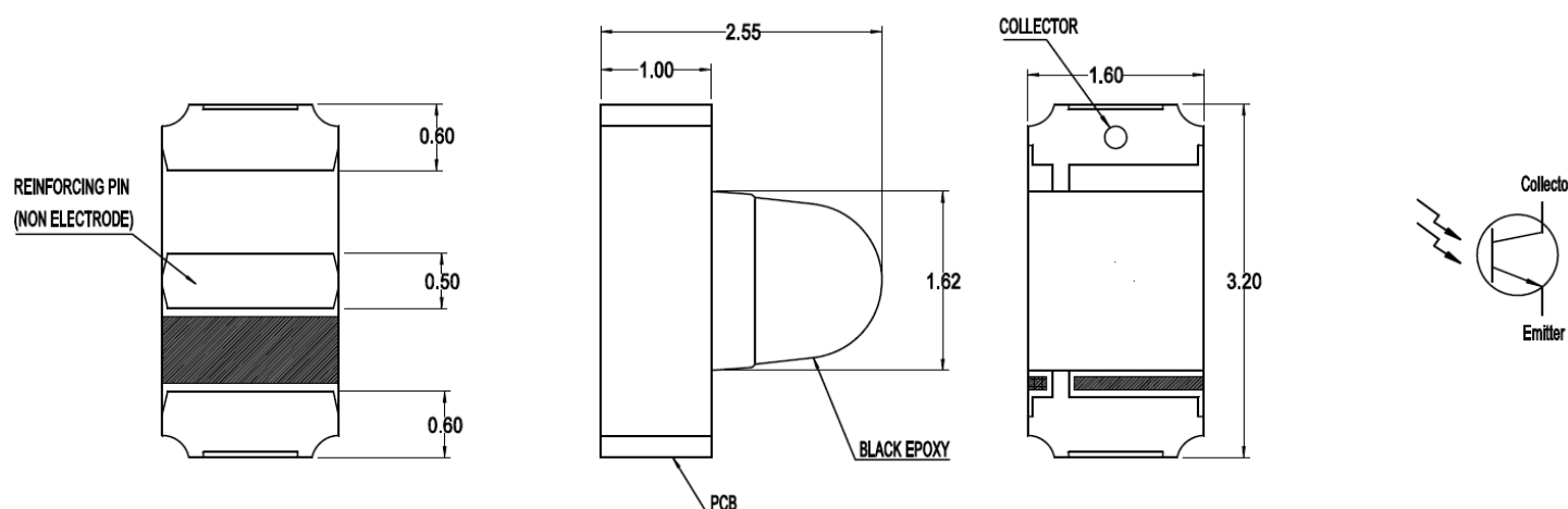
Figure 1: Package Drawing
