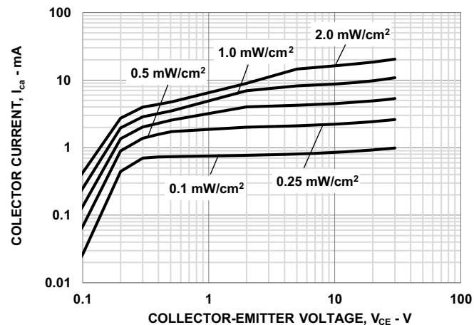
Figure 7: Collector Current vs. Collector-Emitter Voltage for HLPT-B3G0
