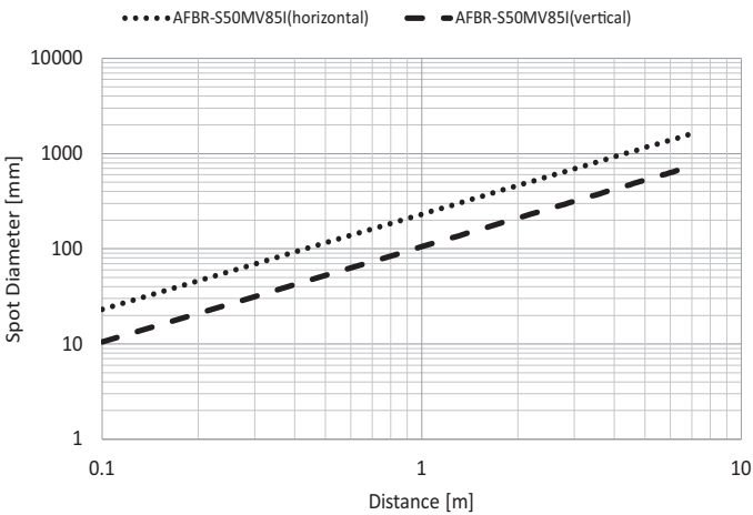
Figure 21: Typical Spot Diameter [mm] over Distance [m]
