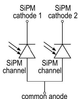
SiPM array
