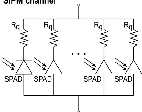
SiPM channel
