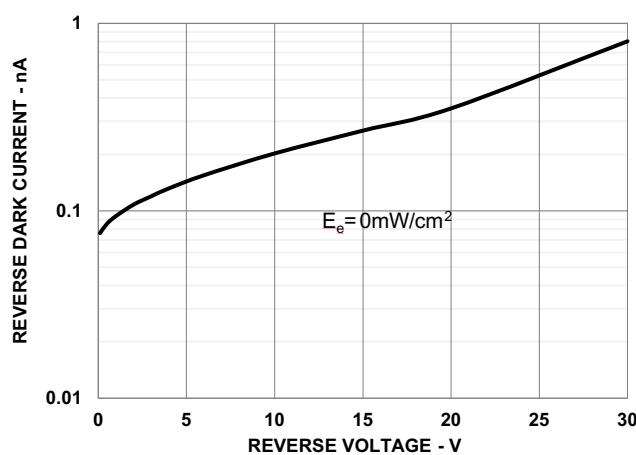
Figure 5: Reverse Dark Current vs Reverse Voltage
