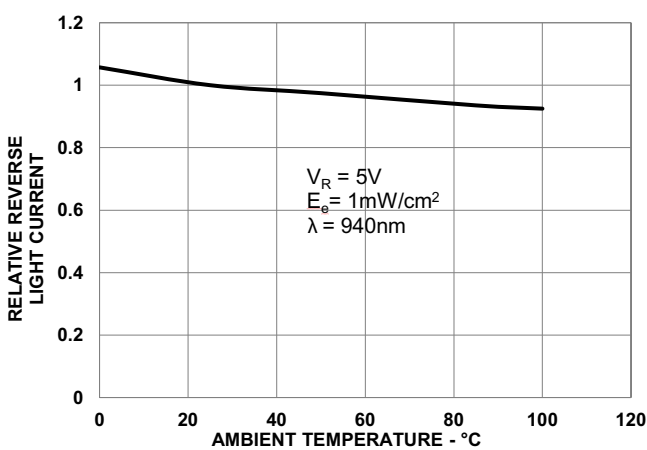
Figure 7: Relative Reverse Light Current vs Ambient Temperature
