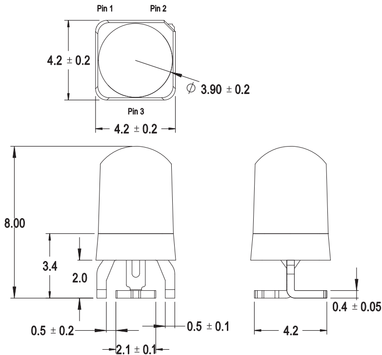
Figure 1: Package Drawing
