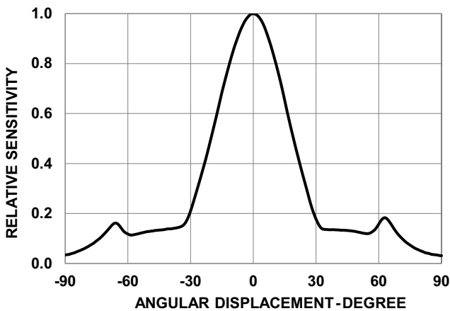
Figure 3: Relative Sensitivity vs. Angular Displacement Angle
