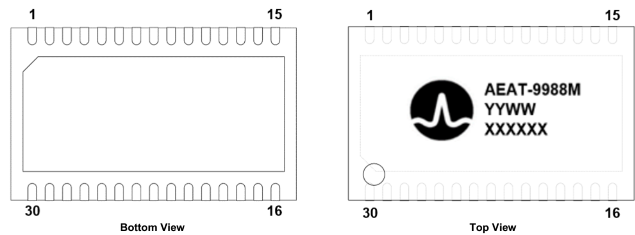
Figure 2: Pin Configuration
