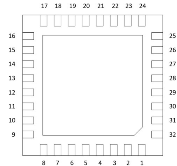
Figure 2 Pin Configurations
