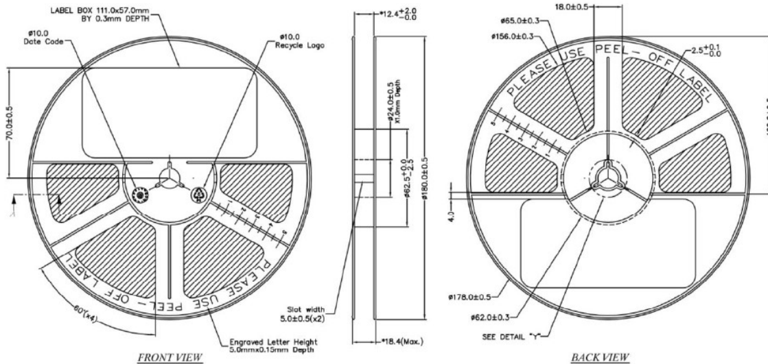
Figure 10 Reel Dimensions
