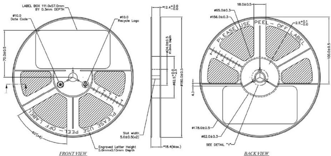
Figure 7: Reel Dimensions
