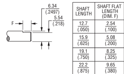
Shaft End Style C
