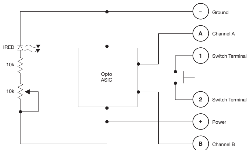
Electrical Block Diagram
