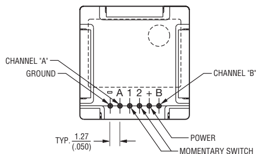
Terminal Diagram
