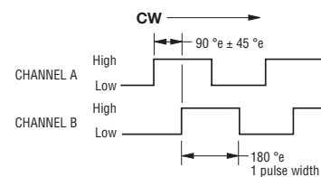
Quadrature Output
