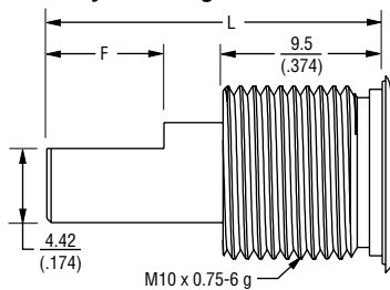
"R" Style Bushing - Flatted Shafts
