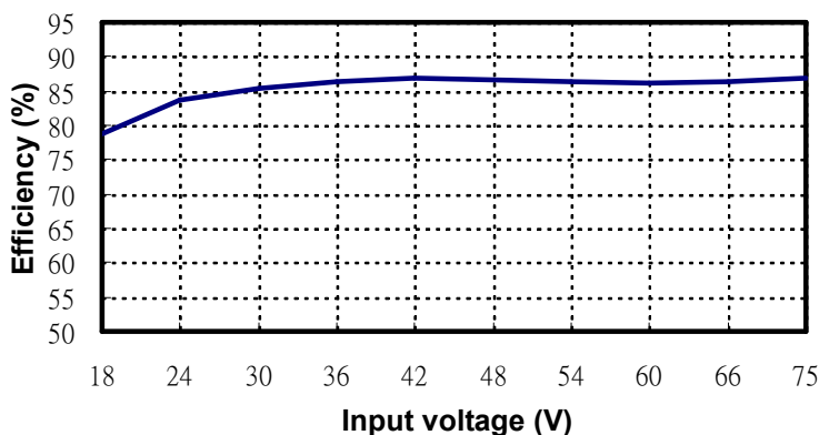
BXC60-48S1W Input voltage vs. Efficiency
