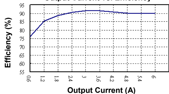
BUC30-48S1 Output Current vs. Efficiency
