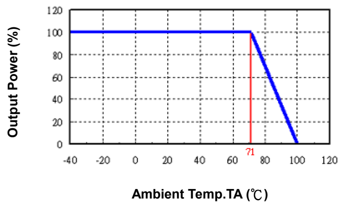
BUB12WSeries Power Derating Curve(5)
