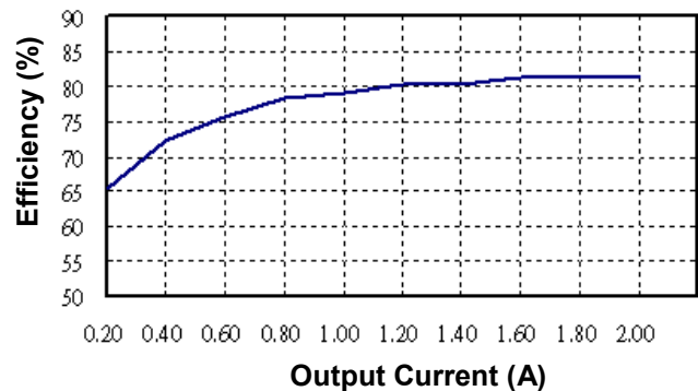
BUB12-48S1W Output Current vs. Efficiency
