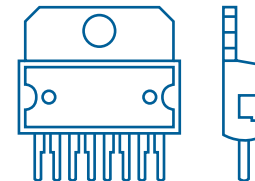
Multiwatt8 (in-line)
