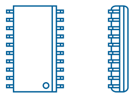
SOIC24w (7.5 mm × 15.4 mm)
