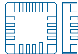
CLCC16 (8 mm × 8 mm)
