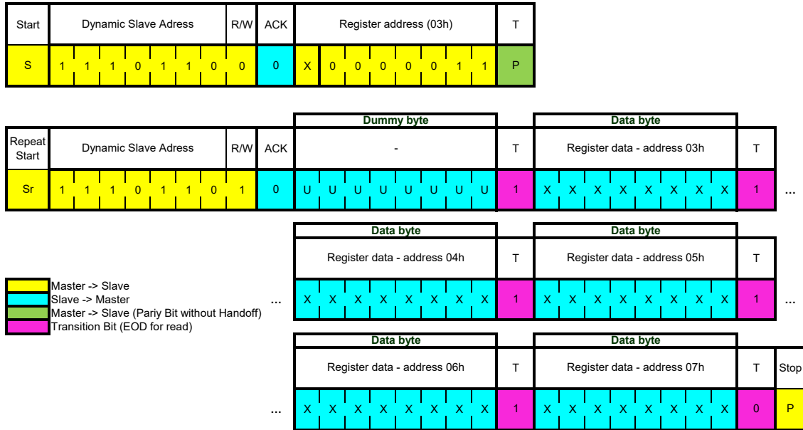
Figure 44: Multi-byte read protocol of I3C with repeated start
