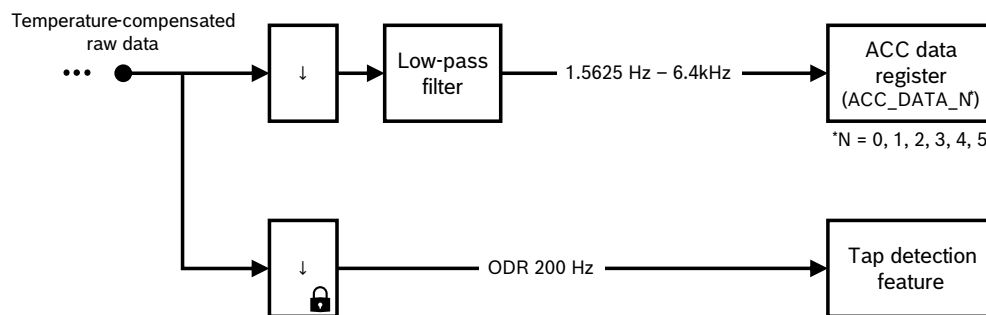
Figure 21: Data path of tap detection
