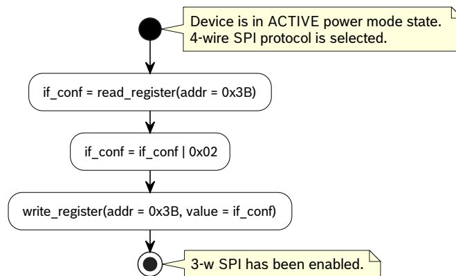
Figure 2: Configure the SPI 3-wire interface
