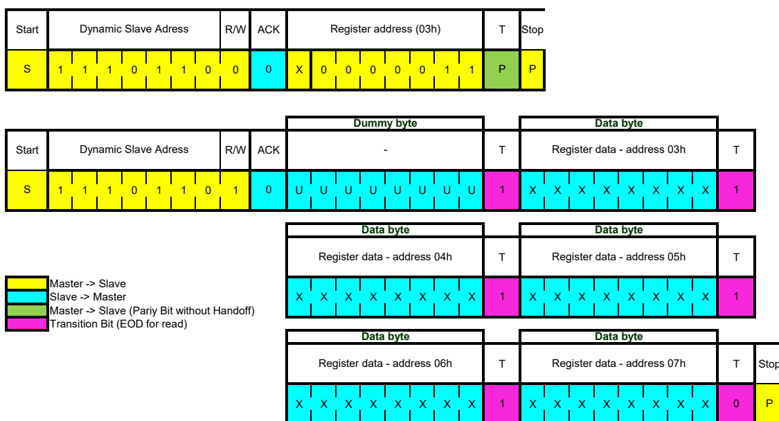
Figure 49: Multi-byte read protocol of I3C with stop-start
