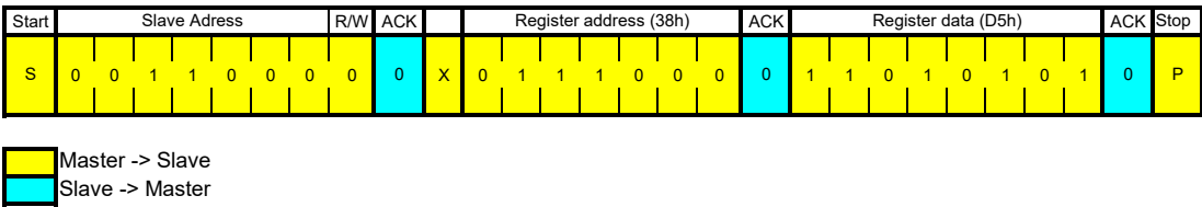
Figure 42: Single-byte write operation of I²C
