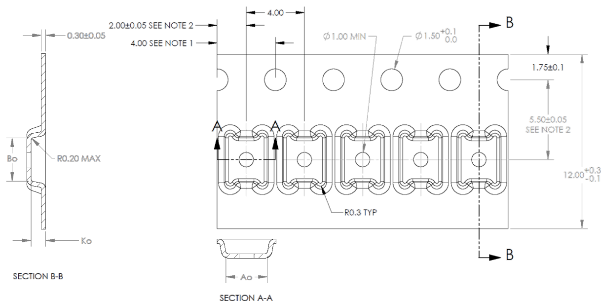
Figure 35: Tape specification
