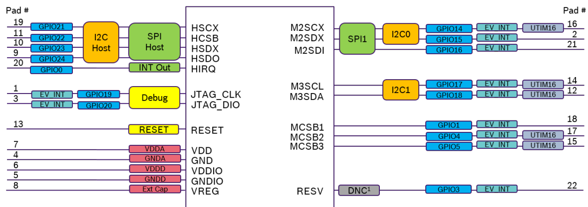
Figure 2: Pinout BHA260AB
