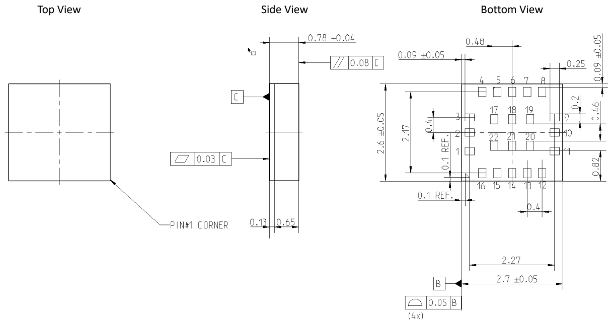
Figure 26: Outline dimensions
