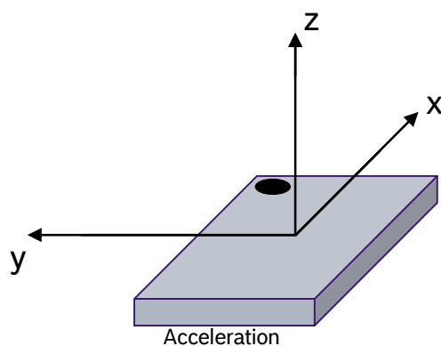
Figure 27: Sensing Axes
