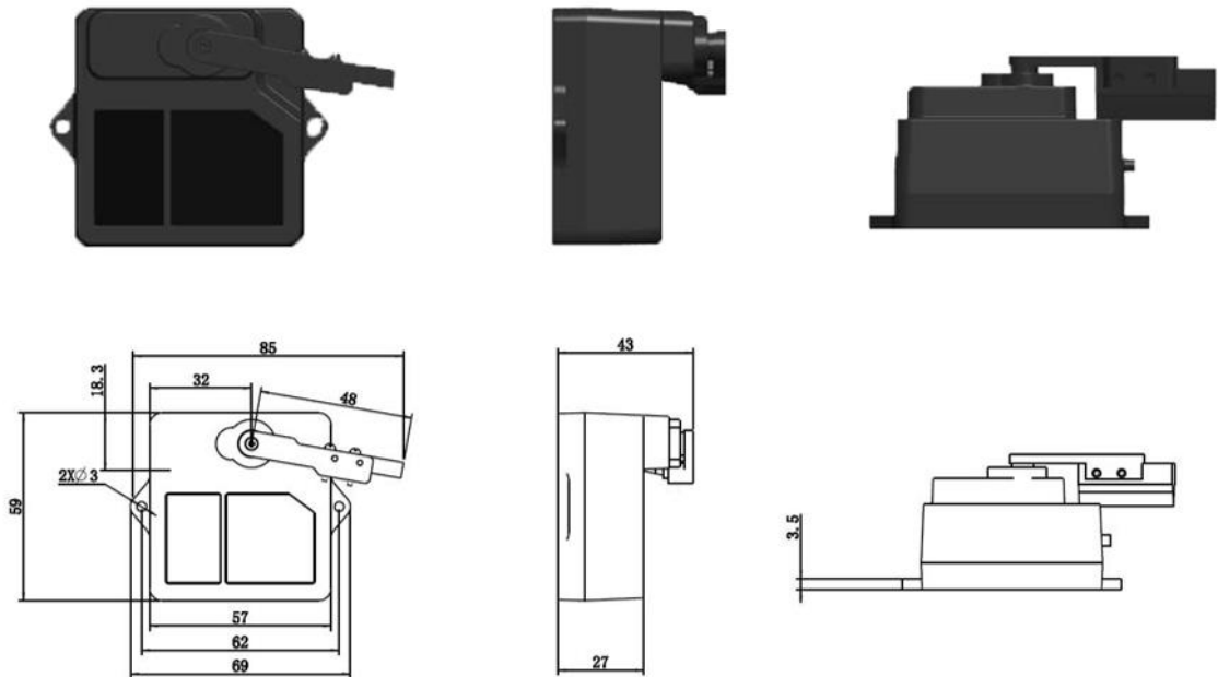
Figure 1 Dimension of TF02-Pro-W (Unit:mm)
