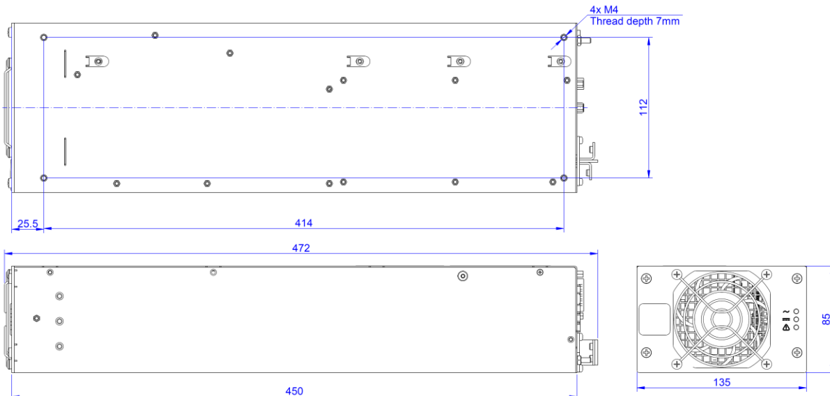
Figure 4. Mechanical Dimensions
