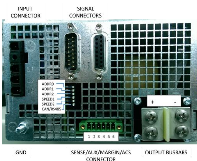
Figure 1. Rear View - Connector Positions
