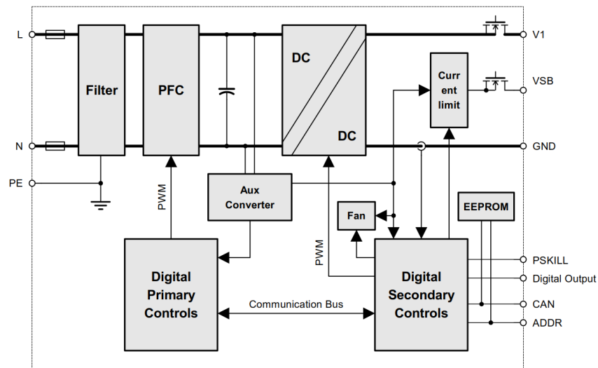
Figure 1. TET4000-48-069RAS441 Block Diagram
