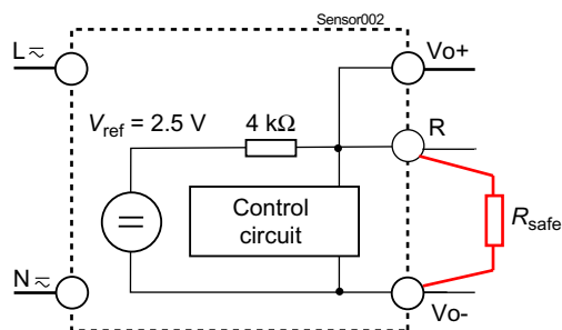
Fig. 1 Block diagram of Power-One converters suited to be controlled by a battery sensor.
