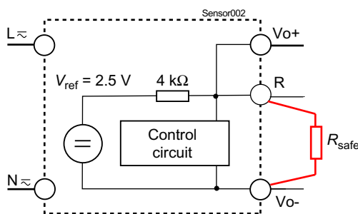
Fig. 5 Connection of R_{\text{safe}} , if standard converter models are used.
