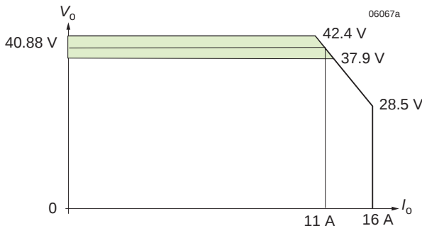
Fig. 11c Output characteristic of LT1840 (typ.). The droop is shown in fig. 12.
