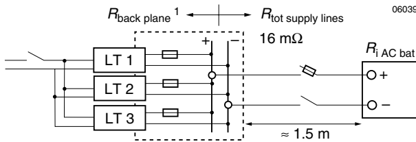
Fig. 10 System set-up
