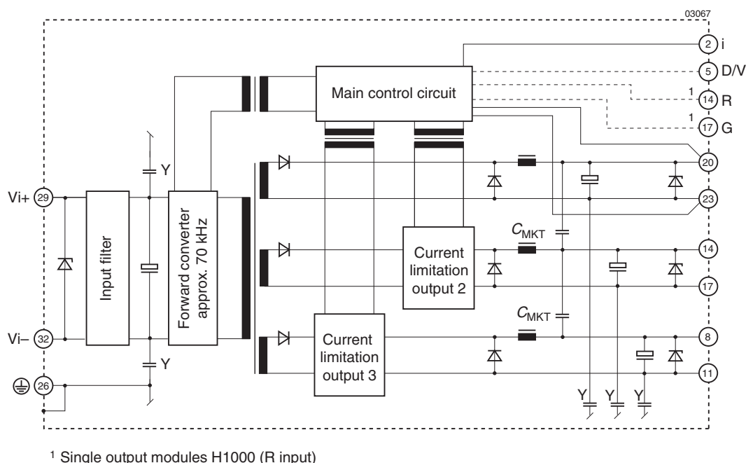
Fig. 1 DC-DC converter block diagram
