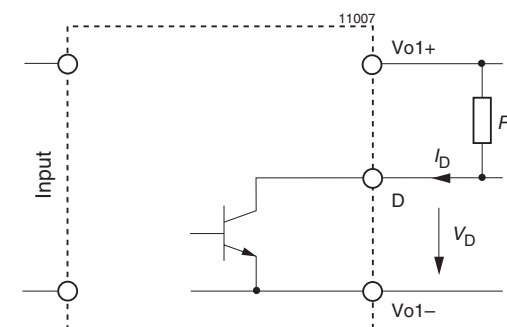
Fig. 16 Options D5 to D8, NPN output
