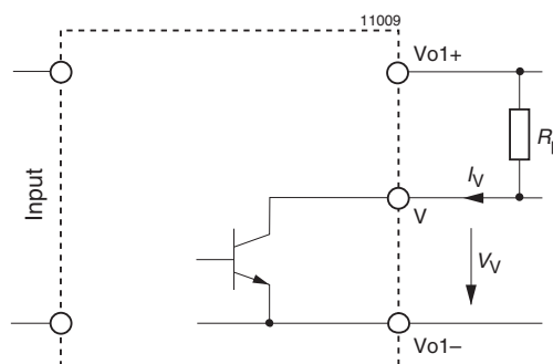
Fig. 19 Output configuration of options V2 and V3
