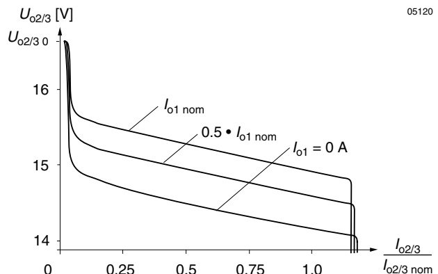
Fig. 4 H2540/H3040: \Delta U_{o2/3} (typ.) versus I_{o2/3} with different I_{o1}
